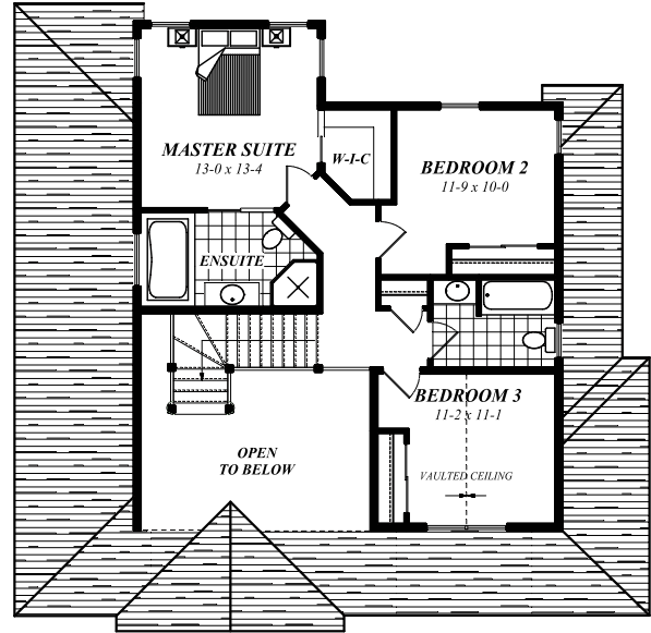
SECOND FLOOR SECOND FLOOR: 830 SF
